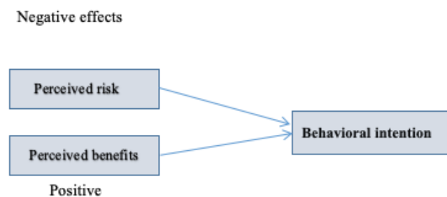
Figure2.1 Diagram of valence theory
